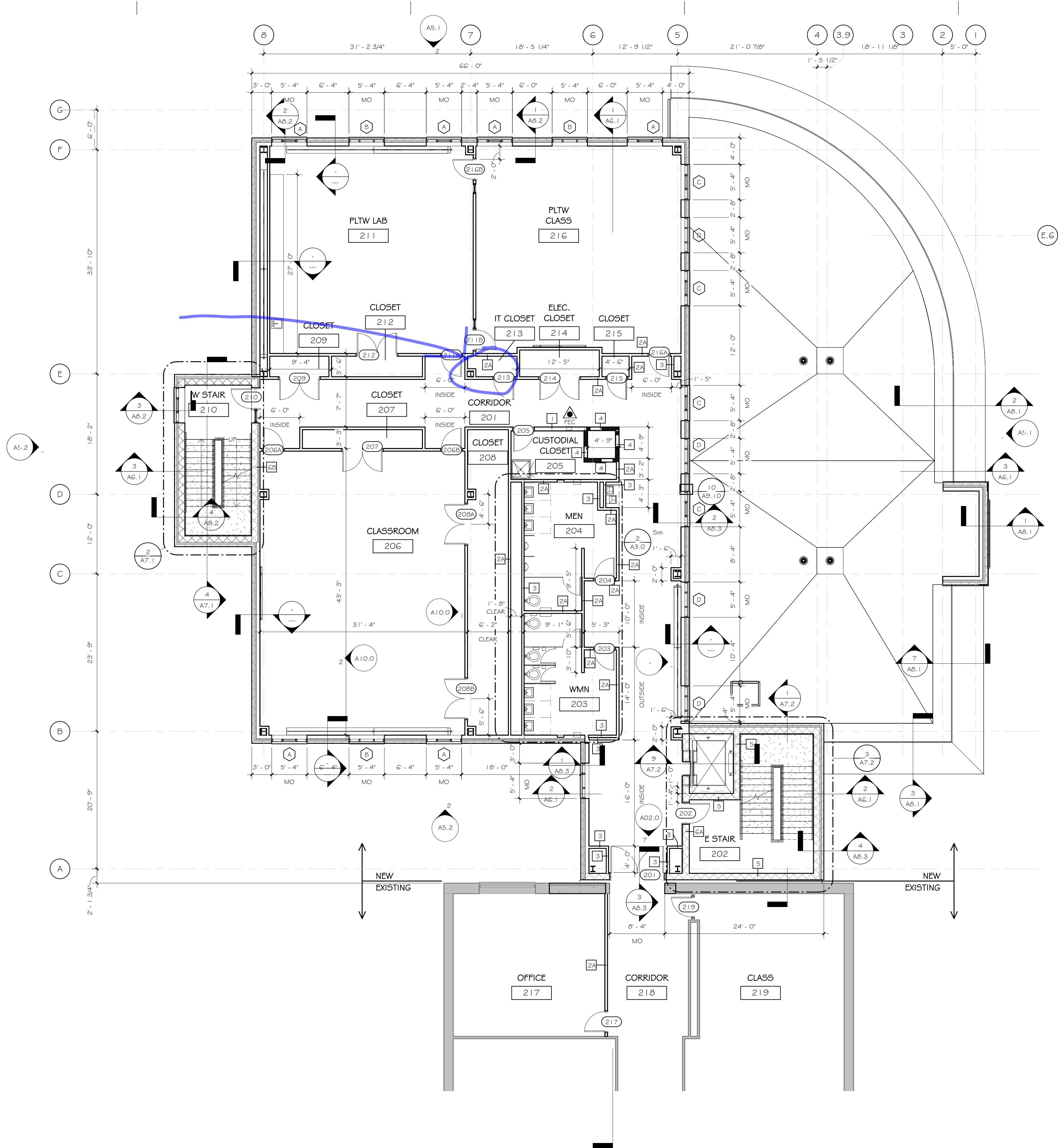
SECOND FLOOR PLAN 1/8" = 1'-0"
