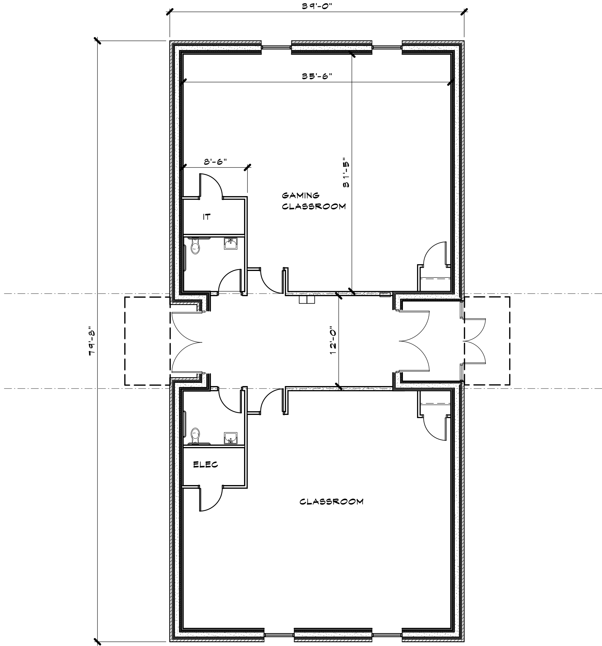
1 PRELIMINARY FLOOR PLAN Scale: 1/8" = 1'-0"
